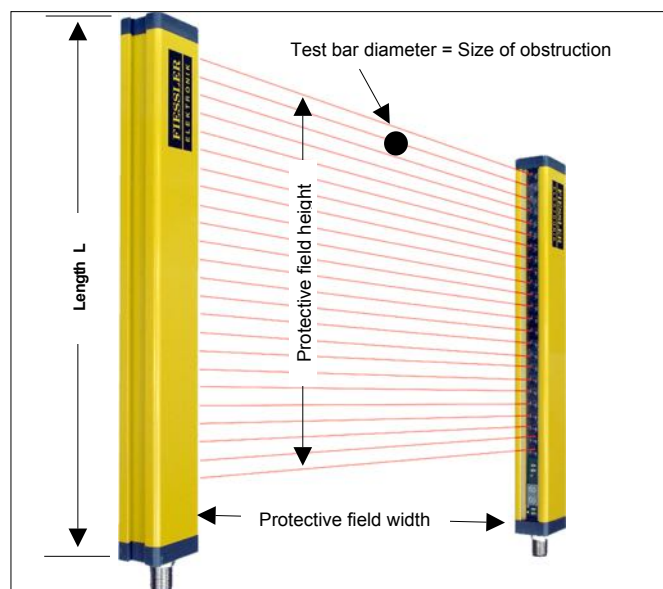
Fig. 5/1: The transmitter and receiver together generate a protective field.
