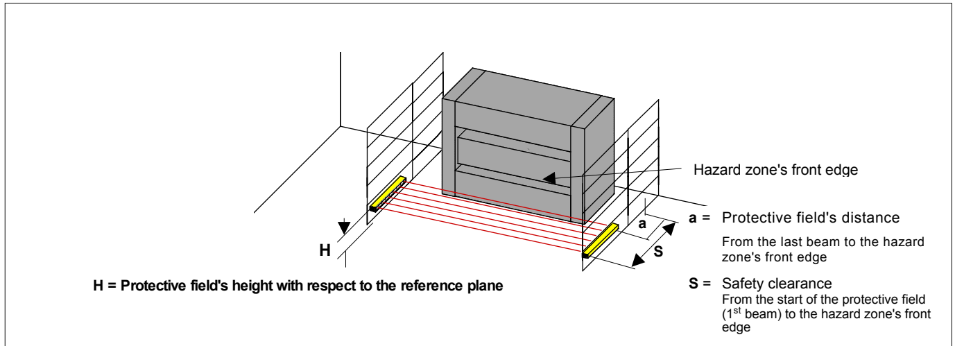
Fig. 13/1: Horizontal safeguarding
