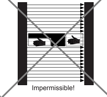
Fig. 25.3: Fixed or floating blanking with partial coverage of the light curtain's blanked section. Additional coverage is necessary.
