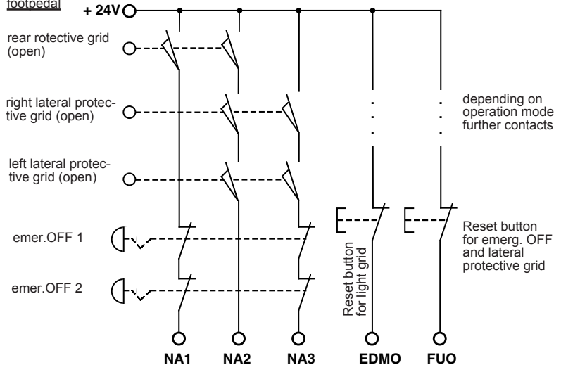
wiring diagram 5b/S.41
