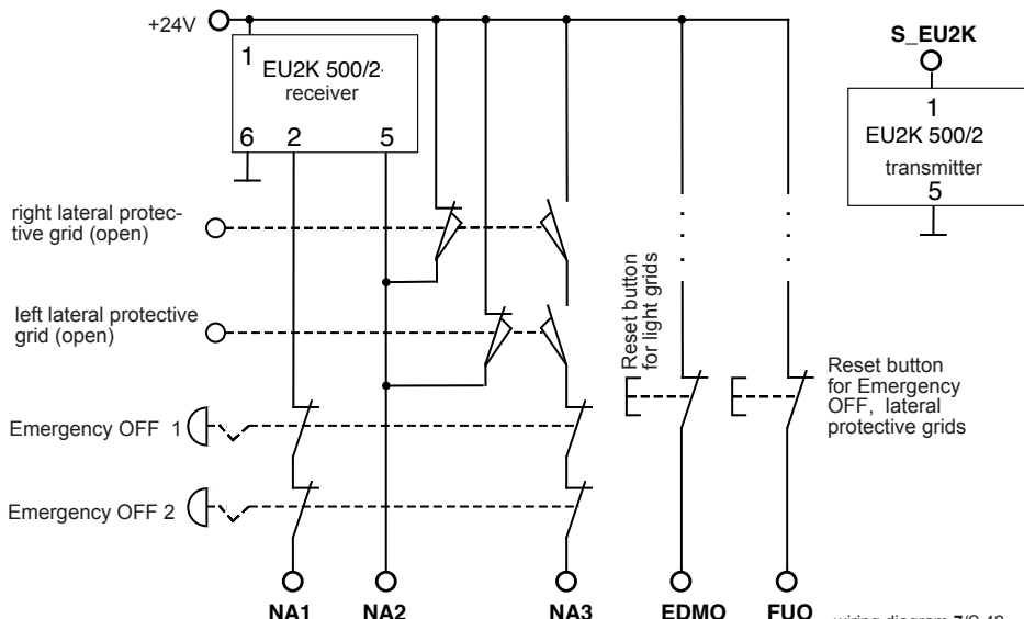
wiring diagram 7/S.42
