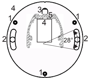
fig 23/1 Base plate
